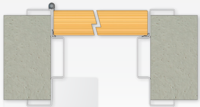
Above: The IS1046si seal is adhered to a clean frame with the bulb section of the seal reversed on the lock and hinge stiles to enable the door to compress against the seal bulb. The seal is fitted to the head of the frame as per the lock stile.
