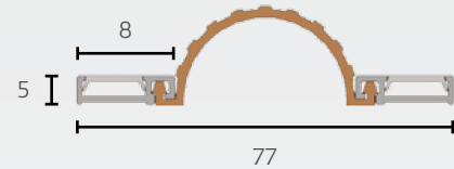
IS9055 Finger Guard Seal - hinge position
