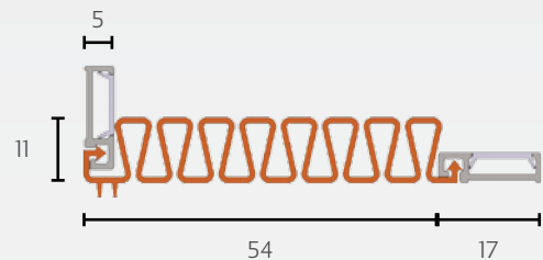
IS9070 Finger Guard Seal
