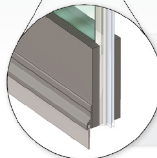
Left: IS7355si seals adhered to 12mm frameless glass pivot door meeting stile.
