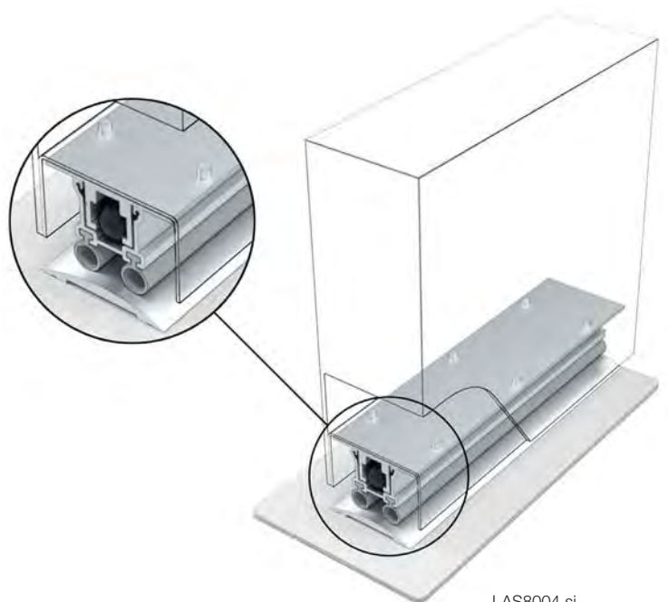
LAS8004 si (Shown with LAS4002)
