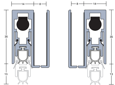
LAS8002G left handed
