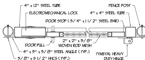
3 GATE SECTION - PLAN Scale: None
