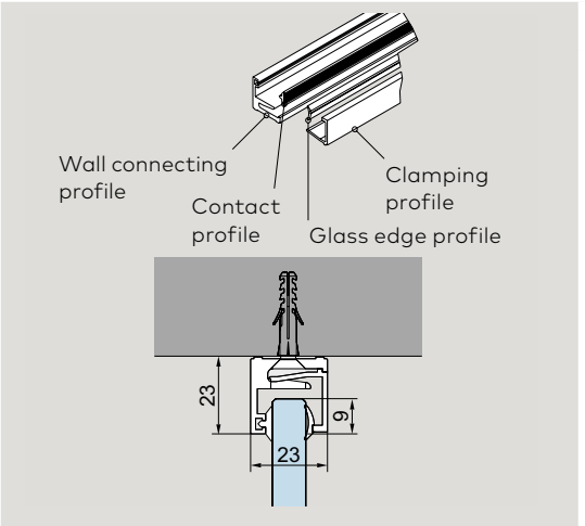
Base profile MR 22
