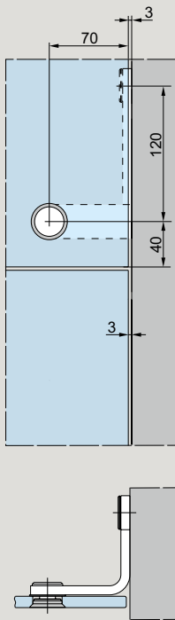
Detail C at wall
