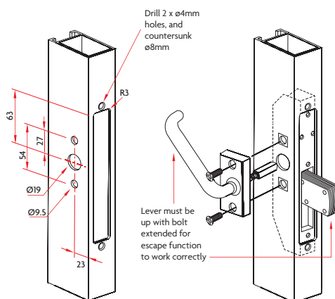
Escape Lever
