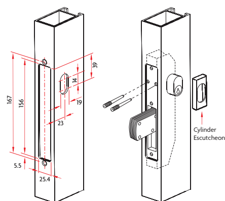
Cylinder/Turn Knob
