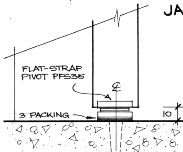
FLOOR DETAIL
