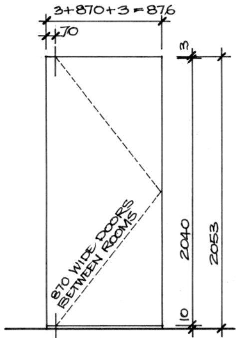
TYPICAL OPENING
