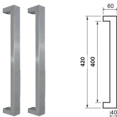
Rectangular Pull Handle
