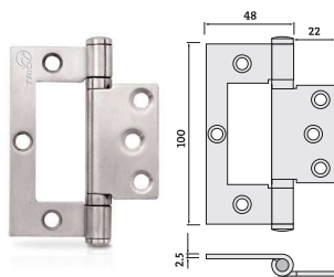
Quick Fit Architectural SS 100 x 70 x 2.5mm | TIMBER FIX
