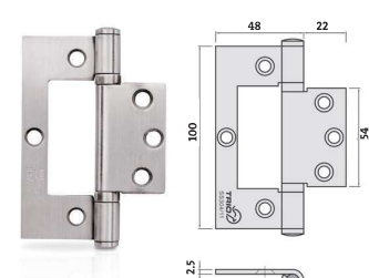
Quick Fit Architectural SS 100 x 70 x 2.5mm | ALUMINIUM FIX
