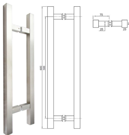
Square Pull Handle 600mm
