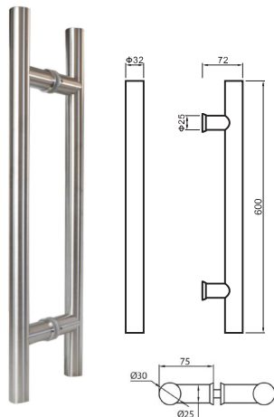
Round Pull Handle 600mm
