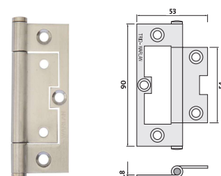
Quick Fit Architectural SS 90 x 53 x 1.8mm | TIMBER FIX
