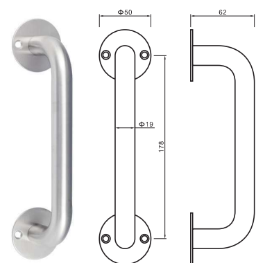
D Handle with plates
