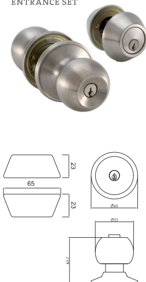
Titan ENTRANCE SET
