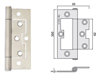
Quick Fit Architectural SS 100 x 65 x 2.0mm | TIMBER FIX
