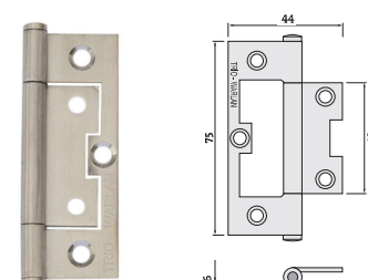
Quick Fit Architectural SS 75 x 44 x 1.6mm | TIMBER FIX
