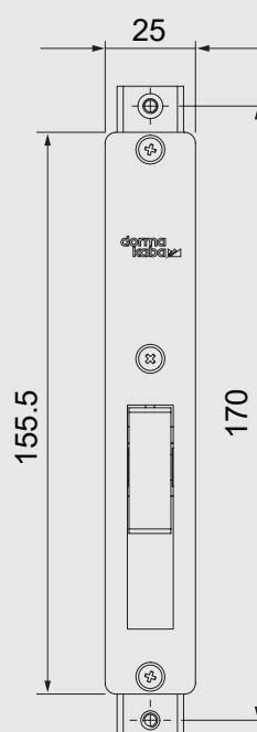
Face plate
