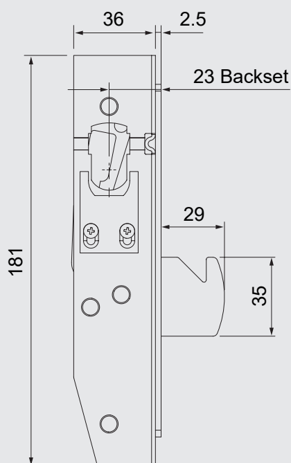
951 lock body
