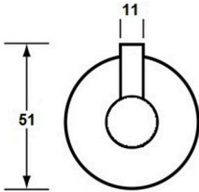
Grub Screw
